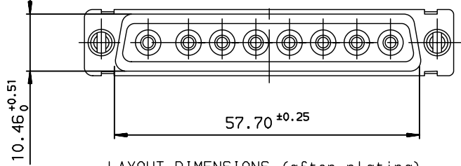
LAYOUT DIMENSIONS (after plating) CONNECTOR SIDE VIEW
